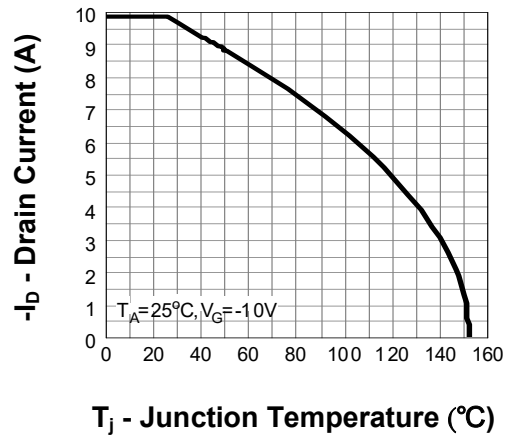
Drain Current
