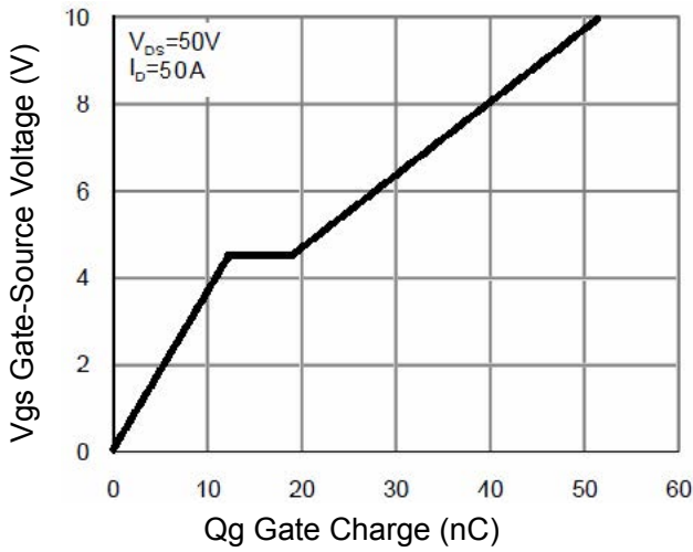
Figure 7 Gate Charge
