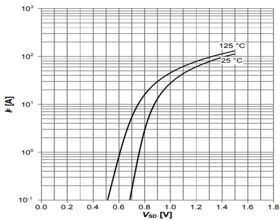
Diagram 11: Forward characteristics of reverse diode
