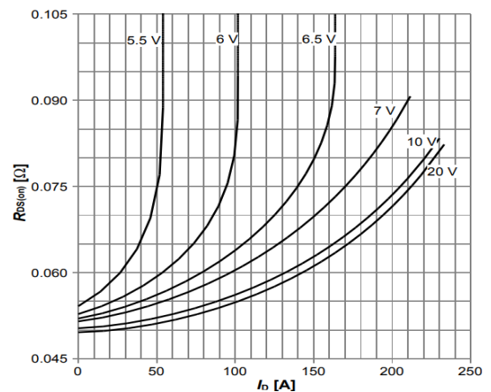
Diagram 12: Typ. Drain-source on-state resistance
