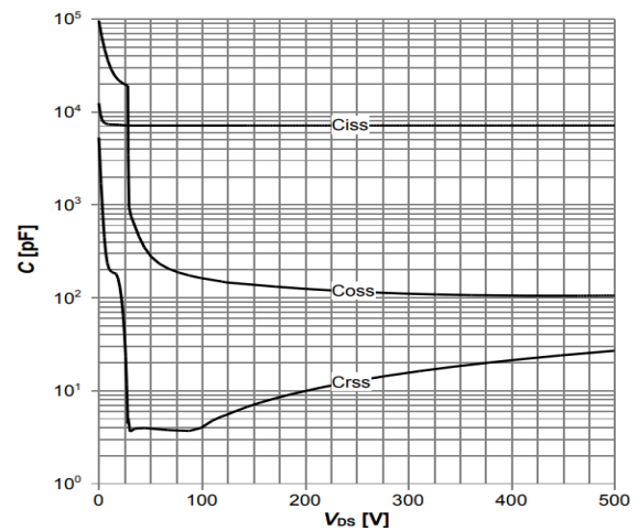
Diagram 6: Typ. capacitances
