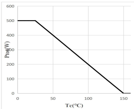
Diagram 9: Typ. Power Dissipation
