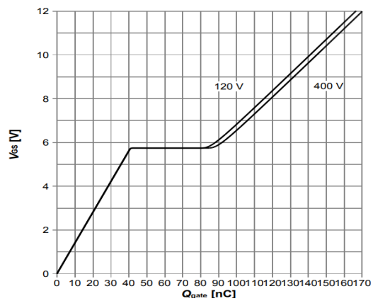
Diagram 4: Typ. gate charge
