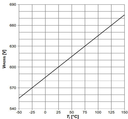
Diagram 5: Drain-source breakdown voltage
