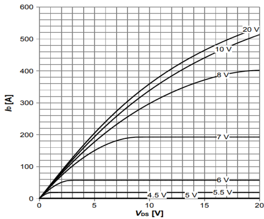
Diagram 1: Typ. output characteristics
