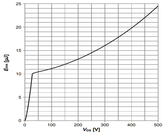
Diagram 2: Typ. Coss stored energy
