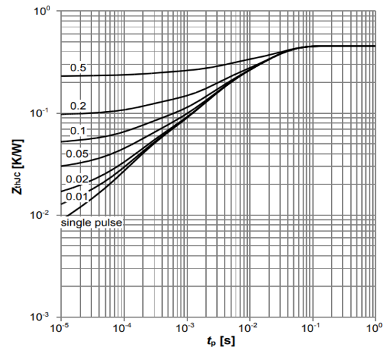
Diagram 10: Max. transient thermal impedance
