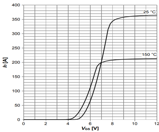
Diagram 3: Typ. transfer characteristics
