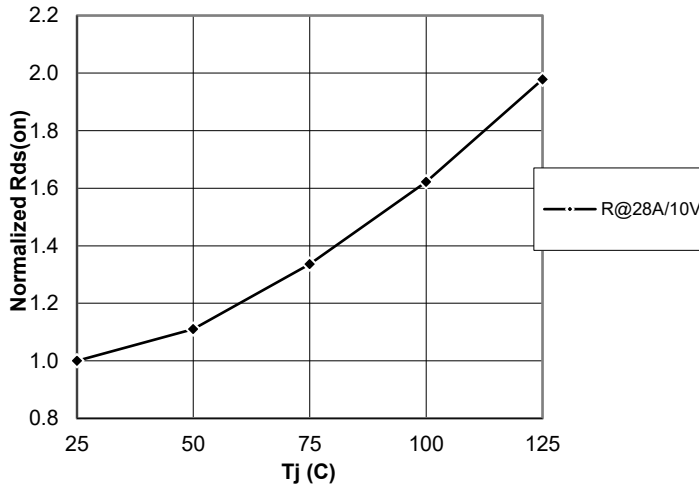
Diagram 7: Typ. On-Resistance vs. Junction Temperature
