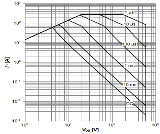
Diagram 8: Safe operating area T c =25 °C, TO247
