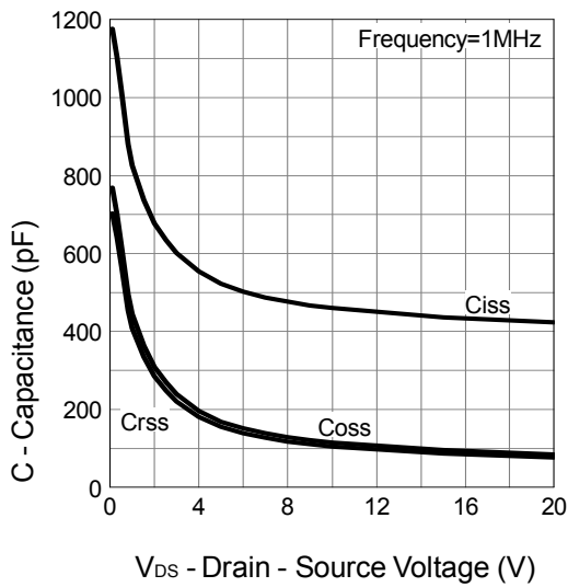
Capacitance
