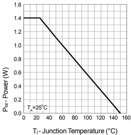
Power Dissipation
