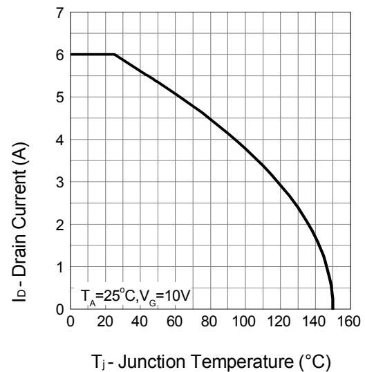
Drain Current
