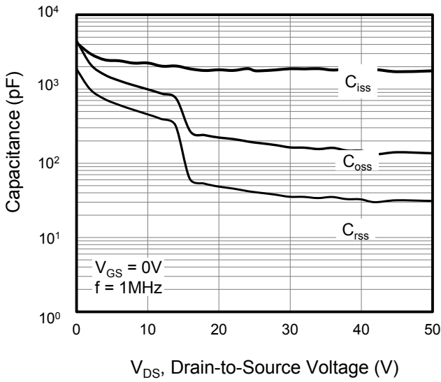
Figure 7. Capacitance
