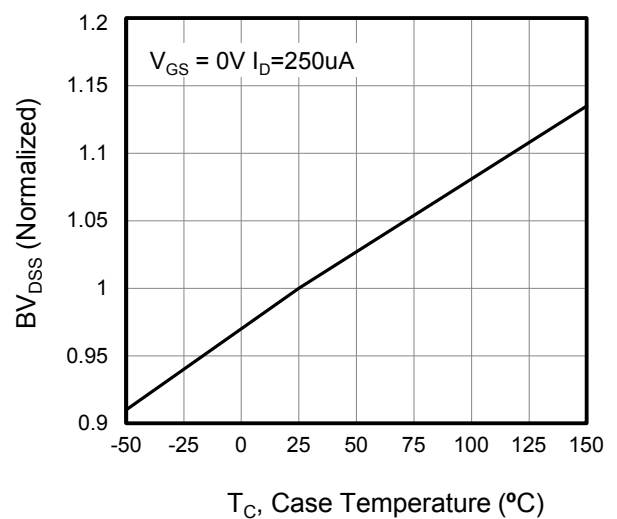
Figure 4. BV_{DS(sat)} Variation vs. Temperature
